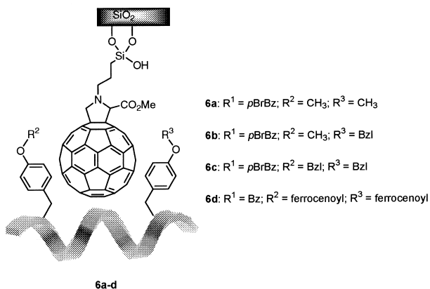
Scheme 6 Supramolecular complex between a silica grafted Fpr and a series of Aib-rich nonapeptides.
