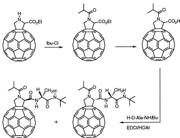
Scheme 3 Synthesis of diastereomeric (Ibu)-L,D-Fpr-D-Ala-NHtBu dipeptides.
